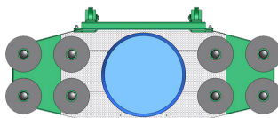
Plan View showing one barrel of additive and eight rolls of bale film
