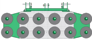
Plan View showing twelve rolls of bale film
