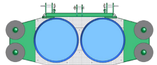
Plan View showing two barrels of additive and four rolls of bale film
